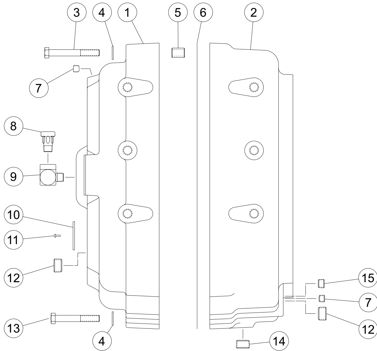
Figure P.9 - TC-200 Housing Parts
